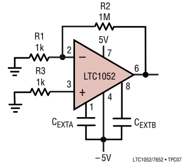
Broadband Noise Test Circuit (TC2)
