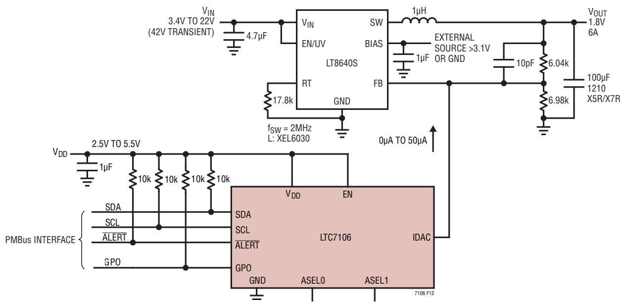
Figure 12. Margining a LT8640S from 1.8V to 1.5V at 6A
