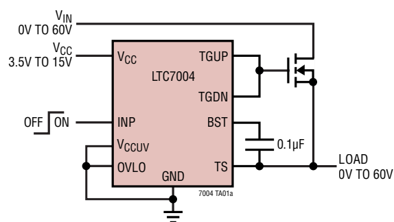
High Voltage, High Side Switch with 100% Duty Cycle
