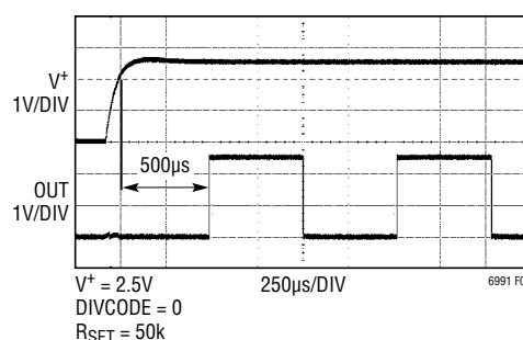
Figure 6. Typical Start-Up
