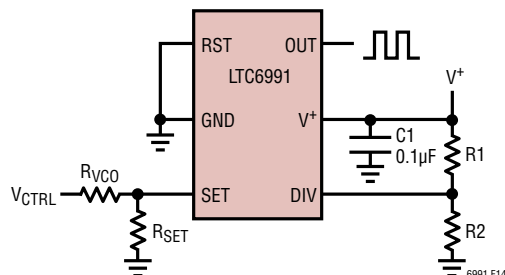
Figure 14. Voltage-Controlled Oscillator
