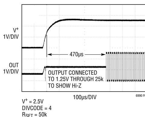
Figure 6. Typical Start-Up
