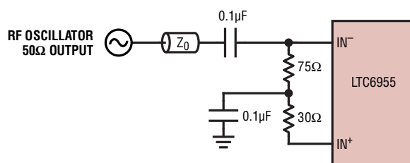
AC-Coupled RF Sine Wave Oscillator ( f_{IN} < 5GHz )
