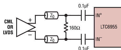
AC-Coupled Differential CML or LVDS ( f_{IN} < 5GHz )
