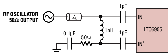
AC-Coupled RF Sine Wave Oscillator ( f_{IN} \geq 5GHz )
