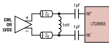
AC-Coupled Differential CML or LVDS ( f_{IN} \geq 5GHz )
