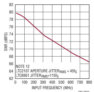
SNR vs Input Frequency of LTC6951 Clocking an LTC2107, f_s = 210\text{Mps} , A_{IN} = -3\text{dBFS}
