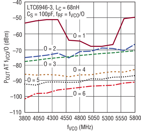
MUTE Output Power vs f_{\text{VCO}} and Output Divide (Single Ended on RF - )
