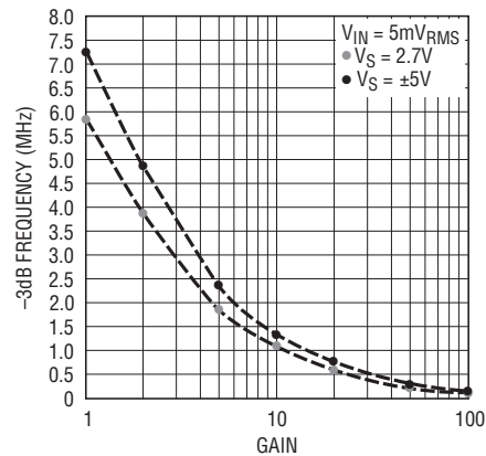
LTC6910-1 -3dB Bandwidth vs Gain Setting
