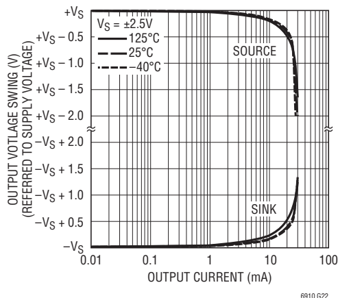
LTC6910-3 Output Voltage Swing vs Load Current
