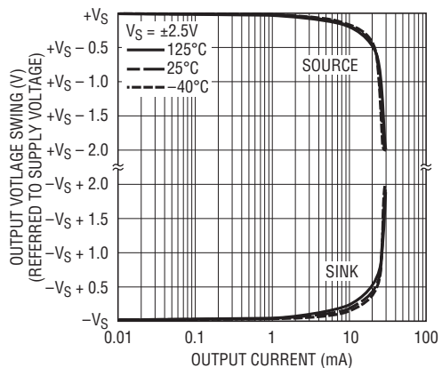
LTC6910-1 Output Voltage Swing vs Load Current
