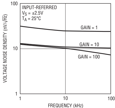
LTC6910-1 Noise Density vs Frequency
