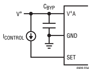
Figure 4. Current Controlled Oscillator
