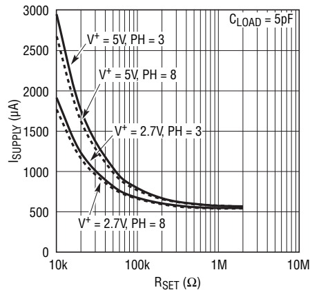
Supply Current vs R_{\text{SET}} (SSFM Enabled)
