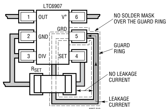
Figure 10. PC Board Layout with Guard Ring
