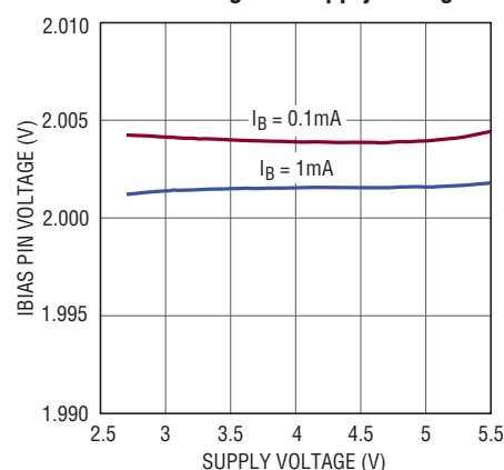
IBIAS Voltage vs Supply Voltage
