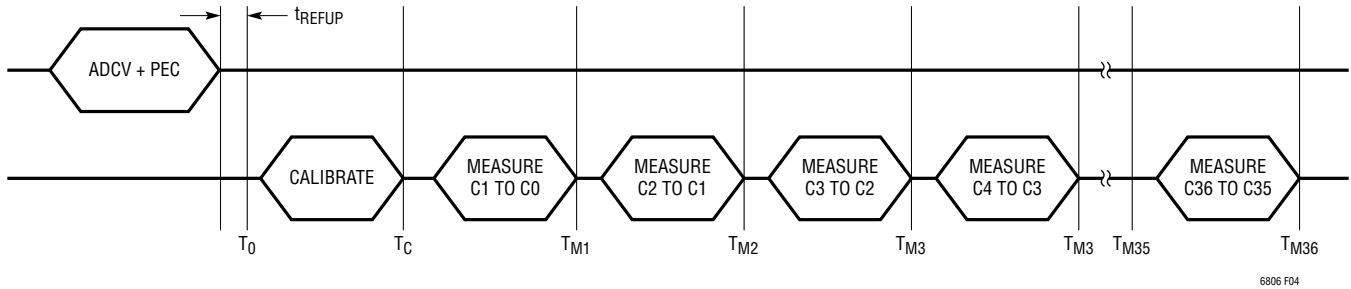
Figure 4. Timing for ADCV Command Measuring All 36 Cells
