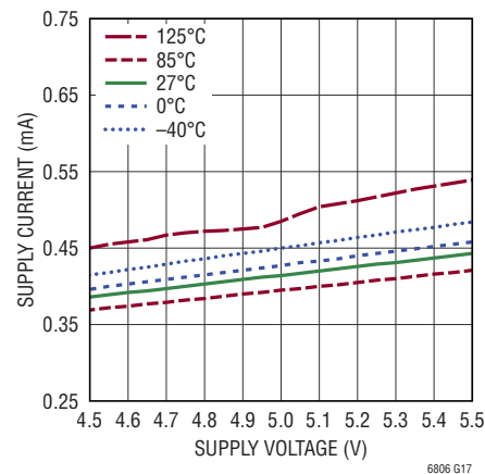
Supply Current vs Supply Voltage, STANDBY Mode
