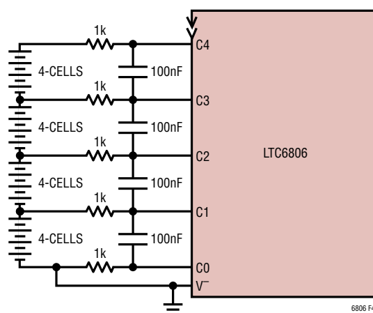
Figure 40. Monitoring Up to Four Cells per Channel
