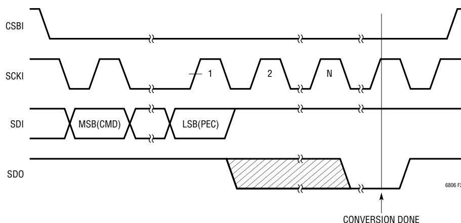
Figure 25. SDO Polling Using the PLADC Command in a Daisy Chain
