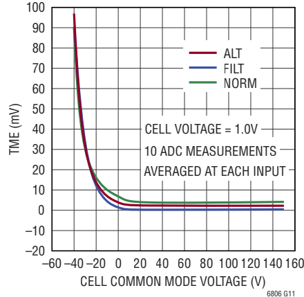
TME vs Cell Common Mode Voltage, LORNG Mode
