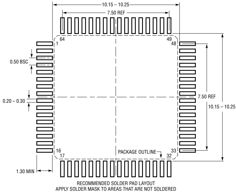
LW Package 64-Lead Plastic LQFP (10mm × 10mm) (Reference LTC DWG #05-08-1539 Rev 0)
