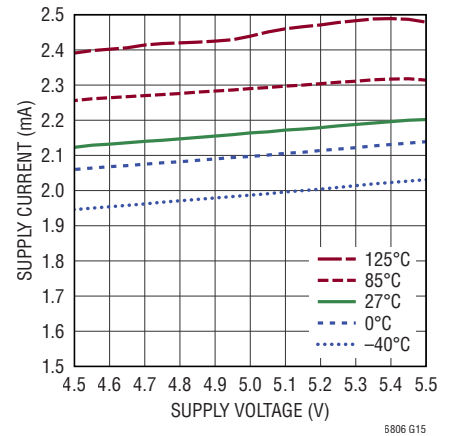
Supply Current vs Supply Voltage, REFUP Mode
