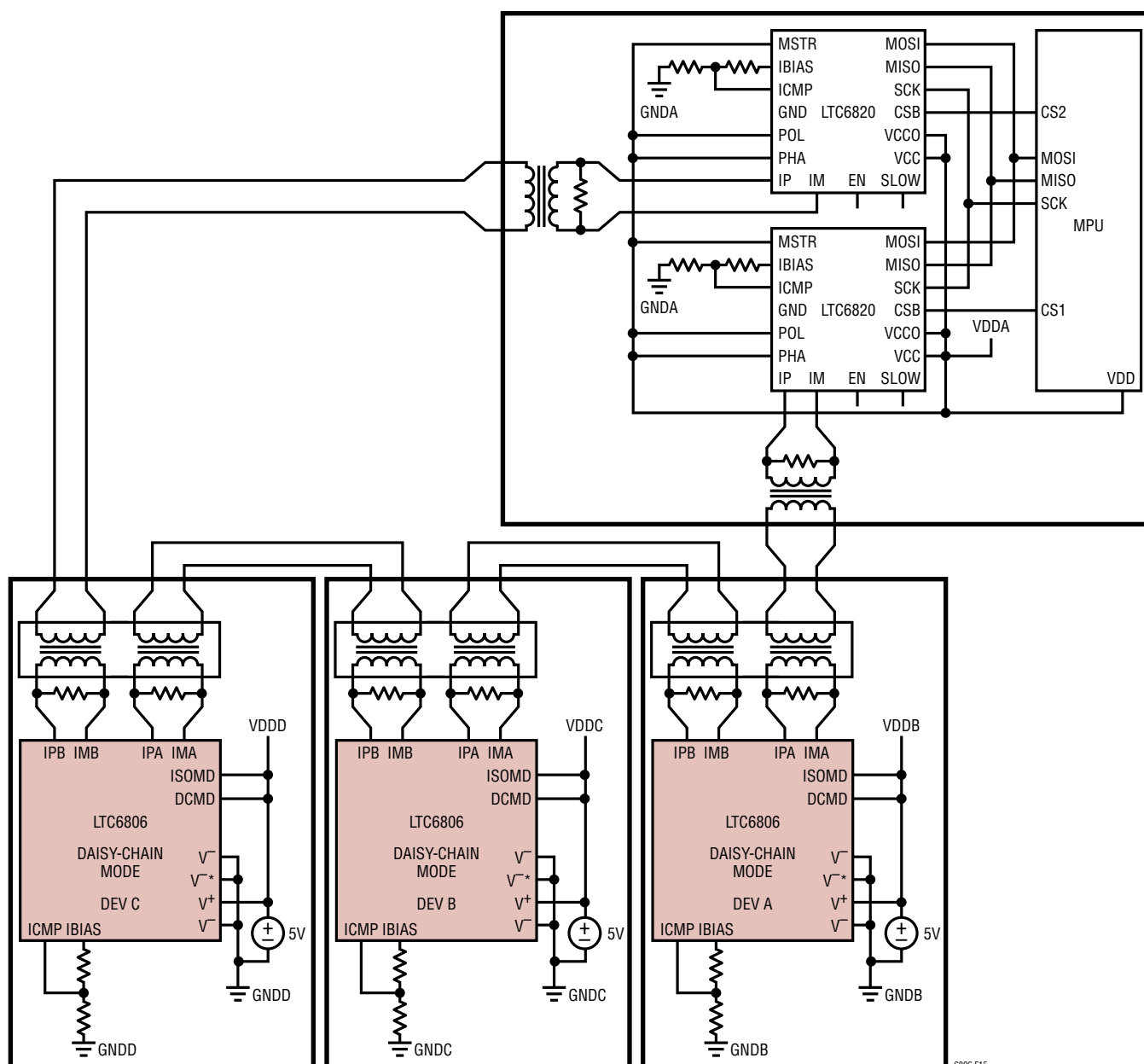
Figure 15. Simplified Transformer Isolated Daisy Chain Configuration with Reversible isoSPI
