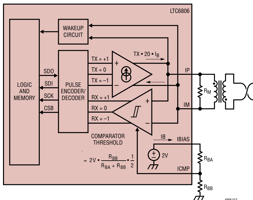
Figure 13. isoSPI Interface
