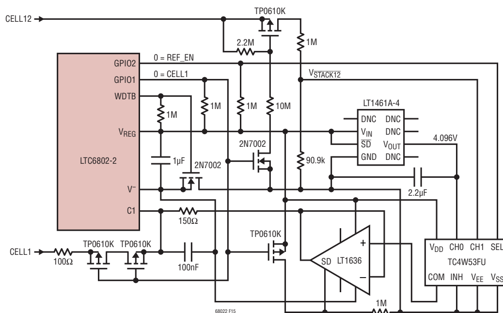
Figure 15. Providing Measurement of Calibration Reference and Full-Stack Voltage Through CELL1 Port
