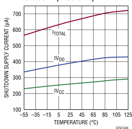
Supply Current vs Temperature, Shutdown (LTC6752-3)
