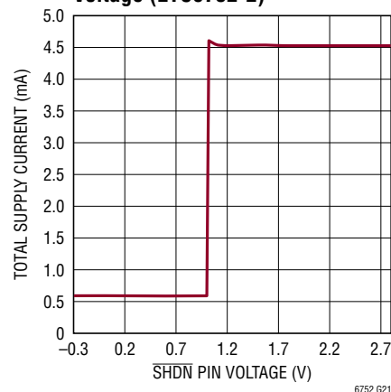
Total Supply Current vs \overline{SHDN} Pin Voltage (LTC6752-2)
