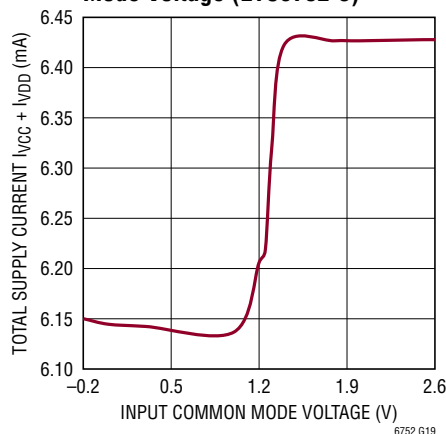
Supply Current vs Input Common Mode Voltage (LTC6752-3)
