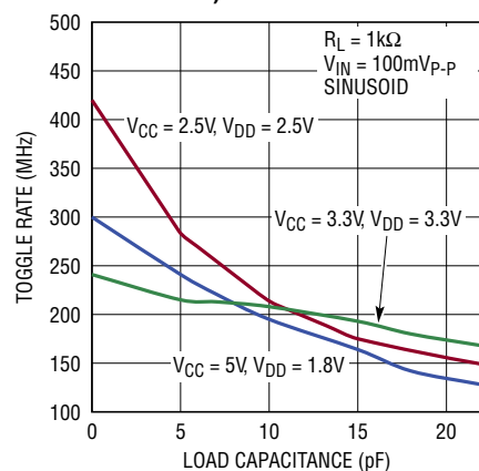
Toggle Rate vs Capacitive Load, (LTC6752/LTC6752-1/LTC6752-2/ LTC6752-4)
