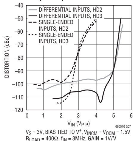
Harmonic Distortion vs Input Amplitude
