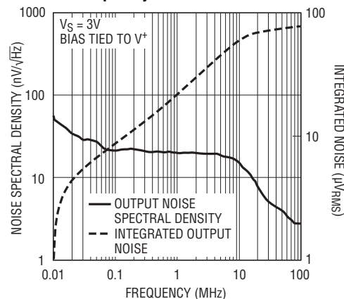
Differential Output Noise vs Frequency
