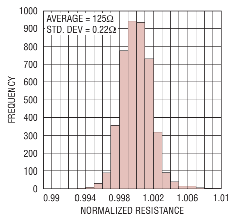
Normalized 125Ω Resistor Trim
