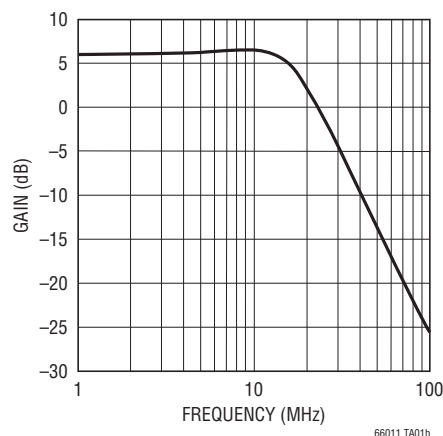
Frequency Response
