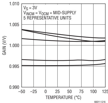
Low Frequency Gain vs Temperature
