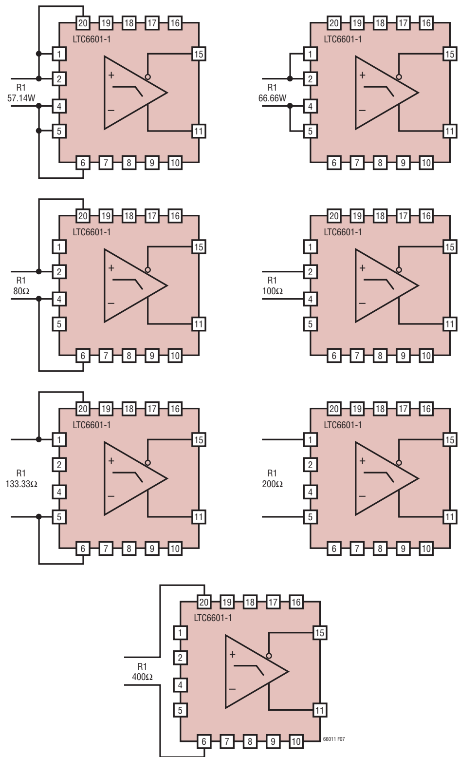
Figure 7. Pin-Strap Hookup for a Particular R1
