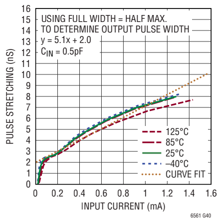
Pulse Stretching C_{IN} = 0.5\text{pF} , Using FWHM
