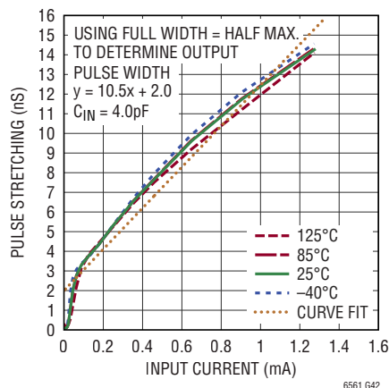
Pulse Stretching C_{IN} = 4.0\text{pF} , Using FWHM
