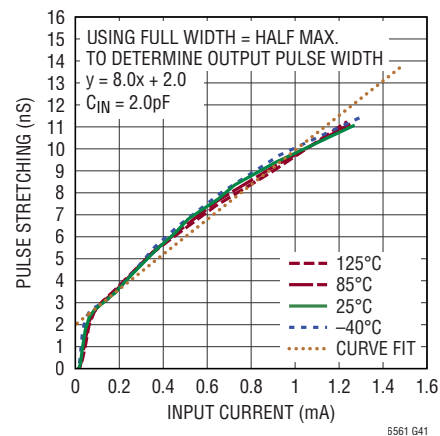
Pulse Stretching C_{IN} = 2.0\text{pF} , Using FWHM
