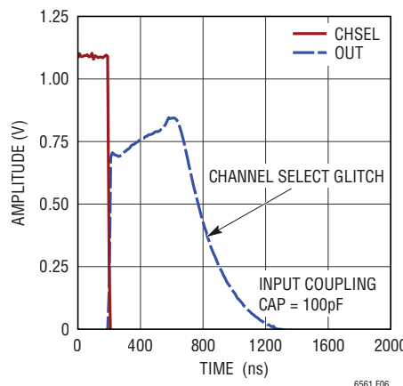
Figure 6. Switching Glitch 100pF
