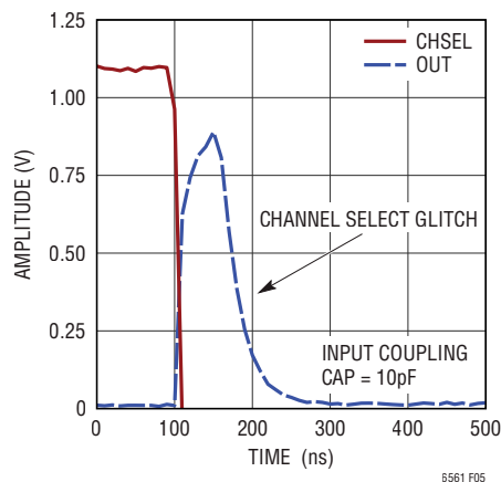
Figure 5. Switching Glitch 10pF
