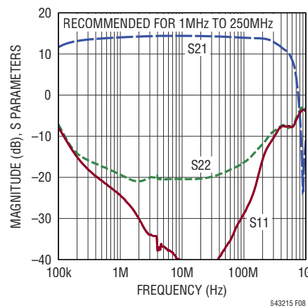
Figure 8. DC2496A with ADT2-1T Baluns
