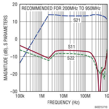
Figure 10. DC2496A with ADTL2-18 Baluns
