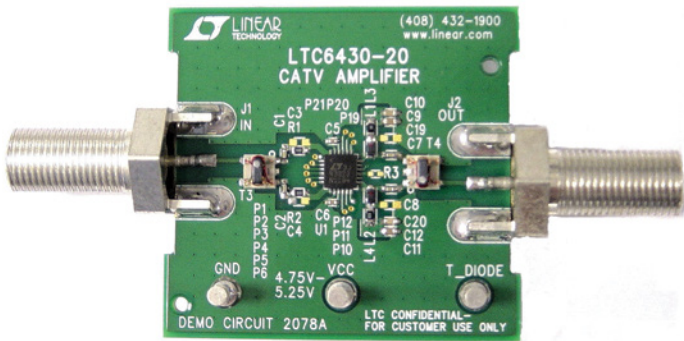
Figure 17. LTC6430-20 CATV Evaluation Board
