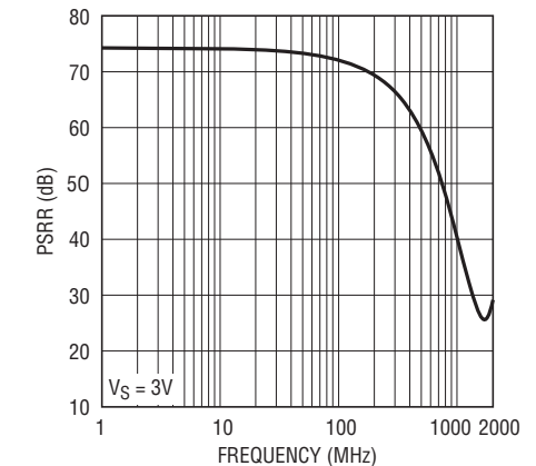
Differential PSRR vs Frequency
