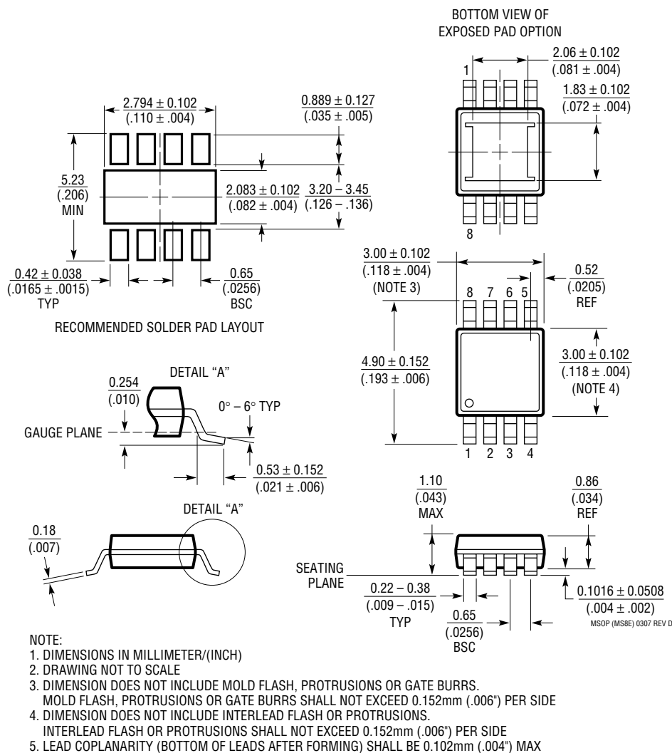
MS8E Package 8-Lead Plastic MSOP (Reference LTC DWG # 05-08-1662)
