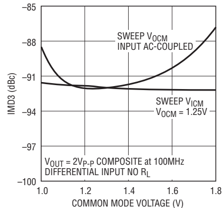
IMD3 vs V_{ICM} and V_{OCM}
