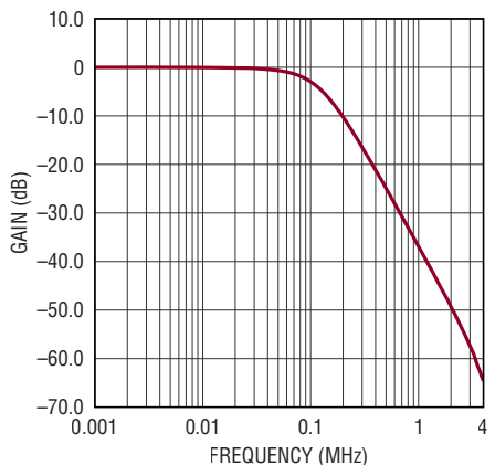
LTC6261 Second Order Butterworth Frequency Response
