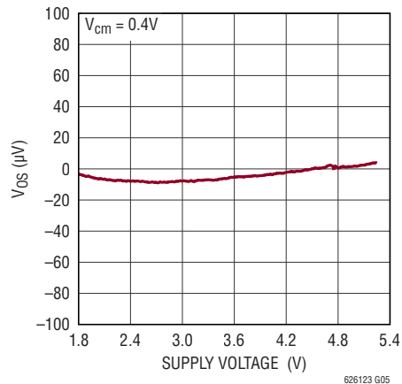
V_{OS} vs Supply Voltage ( 25^{\circ}C )
