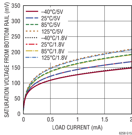
Output Saturation Voltage vs Load Current
