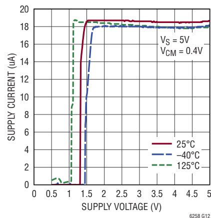
Supply Current vs Supply Voltage per Channel
