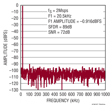
LTC6253-7 Driving LTC2314-14 1024 Point FFT
