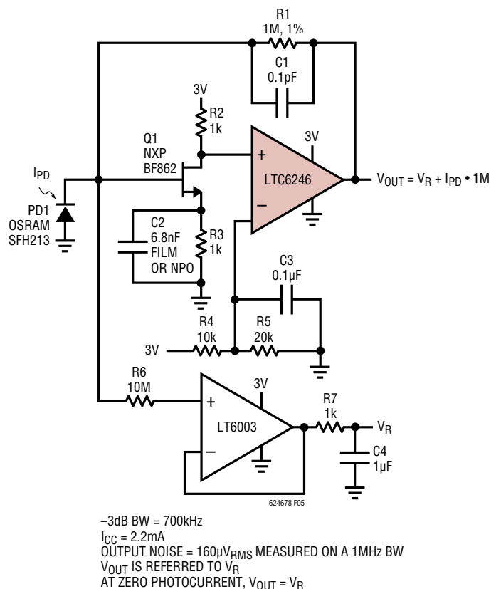
Figure 5. Low Noise Low Power DC Accurate Single Supply Photodiode Amplifier
