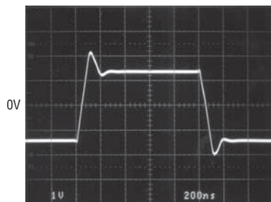
Large-Signal Response
