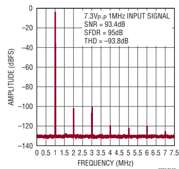
System Performance: 2 x LTC6228 Driving LTC2387-18 8192 Point FFT, -1dBFS f_{\text{SAMPL}} = 15\text{Msps} , f_{\text{IN}} = 1\text{MHz}
