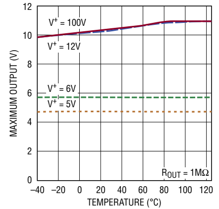
Maximum V_{OUT1} vs Temperature
