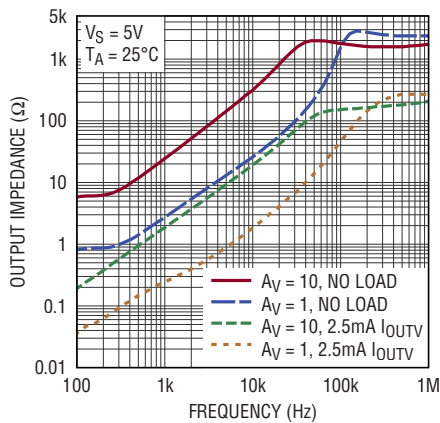
Output Impedance vs Frequency (OUTV)
