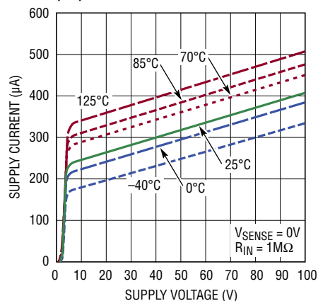
Supply Current vs Supply Voltage ( V^+ )
