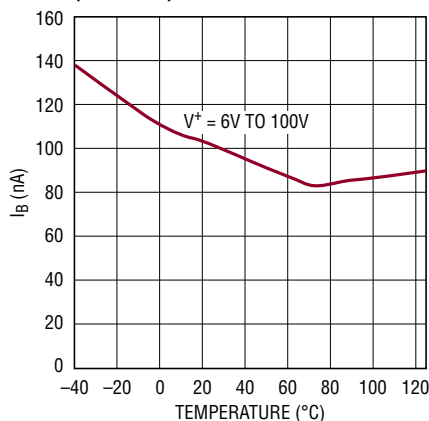
Input Bias Current vs Temperature (+IN, -IN)
