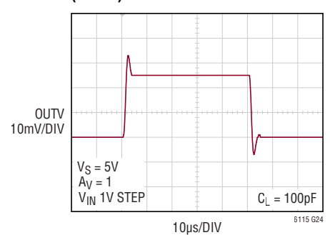
Small Signal Step Response (OUTV)
