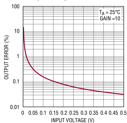
Output Error Due to Input Offset vs Input Voltage
