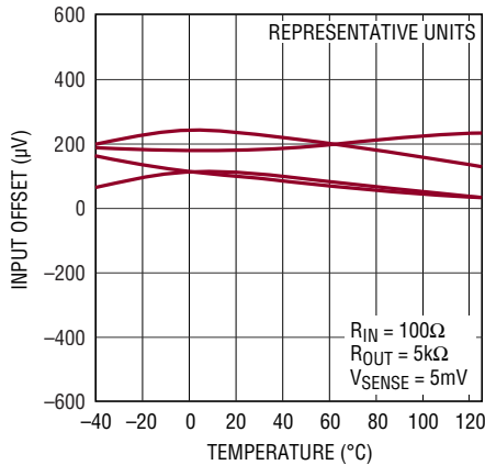
V_{OS} vs Temperature (+IN, -IN)
