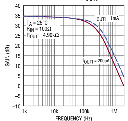
Gain vs Frequency ( V_{OUT1} )
