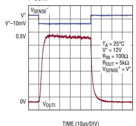
Step Response 0mV to 10mV ( V_{OUT1} )
