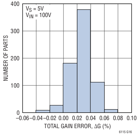
Total Gain Error Distribution
