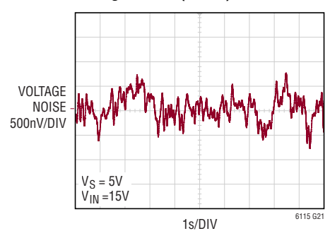
0.1Hz to 10Hz Output Voltage Noise (OUTV)
