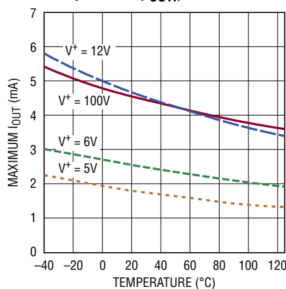
Maximum Output Current vs Temperature ( I_{OUT1} )
