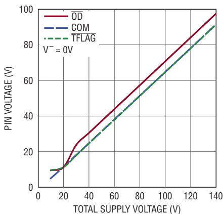
Open-Circuit Voltage of COM, \overline{\text{OD}} , TFLAG
