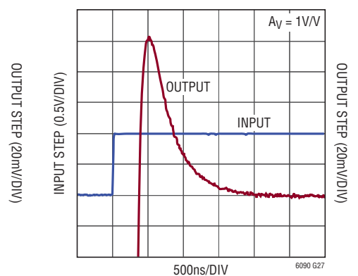
LTC6090 Rising Edge Settling Time
