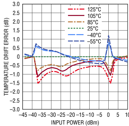
Linearity Error Temperature Variation from 25^\circ C at 5.8GHz
