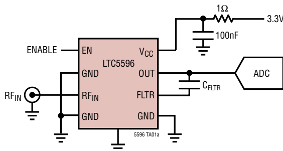
100MHz to 40GHz RMS Power Detector
