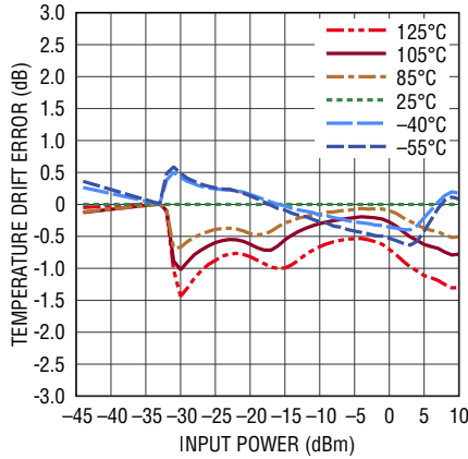
Linearity Error Temperature Variation from 25^\circ C at 50MHz
