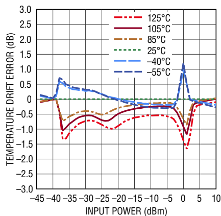
Linearity Error Temperature Variation from 25°C at 24GHz
