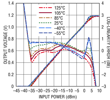
Output Voltage, Linearity Error vs RF Input Power at 100MHz
