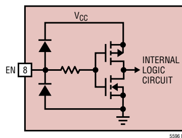
Figure 7. Simplified Schematic of the EN Interface
