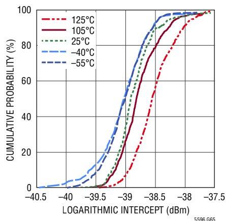
Logarithmic Intercept Cumulative Distribution
