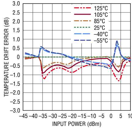
Linearity Error Temperature Variation from 25^\circ C at 100MHz
