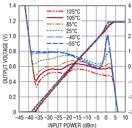
Output Voltage, Linearity Error vs RF Input Power at 10GHz
