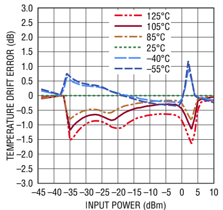
Linearity Error Temperature Variation from 25^\circ C at 15GHz
