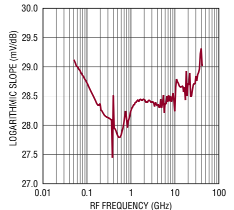
Logarithmic Slope vs Frequency
