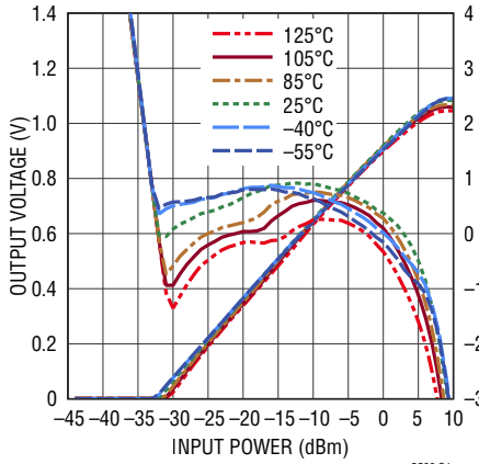
Output Voltage, Linearity Error vs RF Input Power at 50MHz
