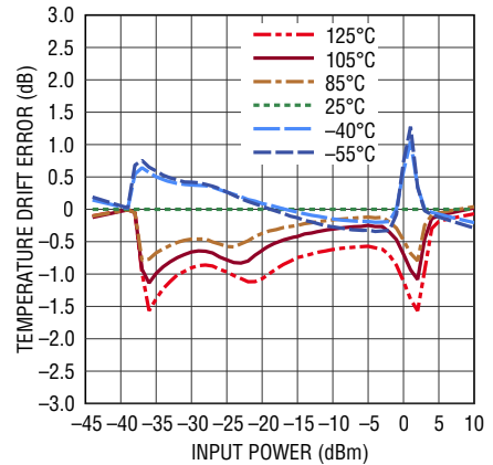
Linearity Error Temperature Variation from 25^\circ C at 7.6GHz
