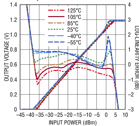
Output Voltage, Linearity Error vs RF Input Power at 12GHz
