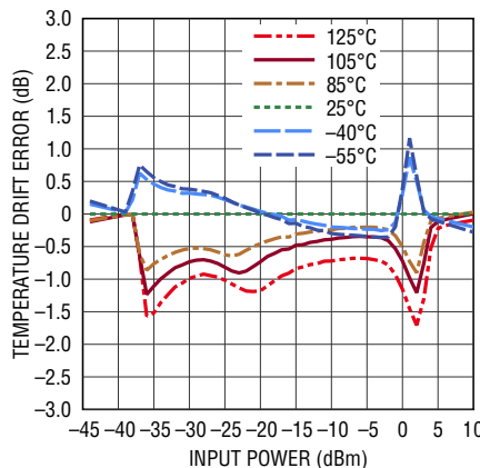
Linearity Error Temperature Variation from 25^\circ C at 12GHz
