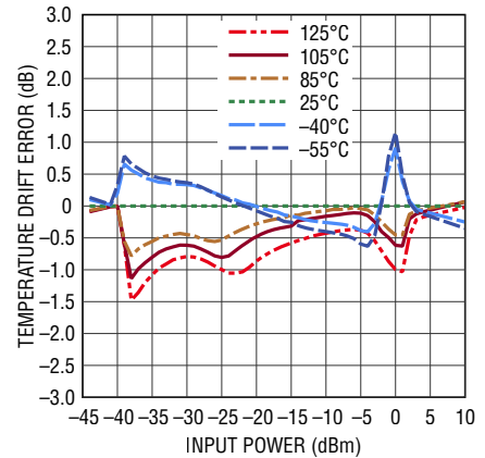
Linearity Error Temperature Variation from 25^\circ C at 500MHz
