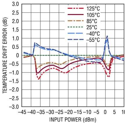
Linearity Error Temperature Variation from 25^\circ C at 2.14GHz
