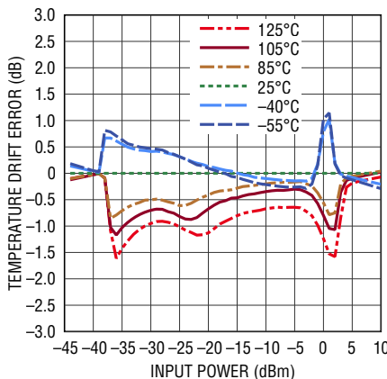
Linearity Error Temperature Variation from 25^\circ C at 10GHz
