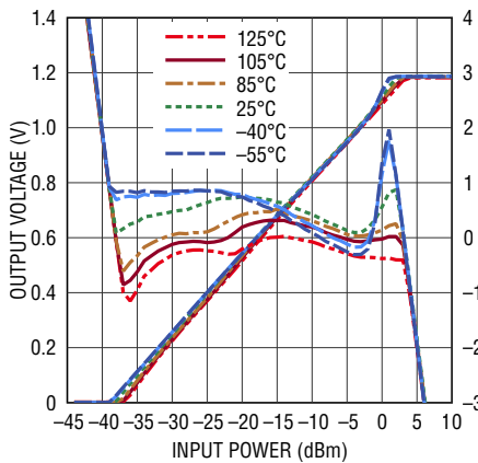
Output Voltage, Linearity Error vs RF Input Power at 2.14GHz
