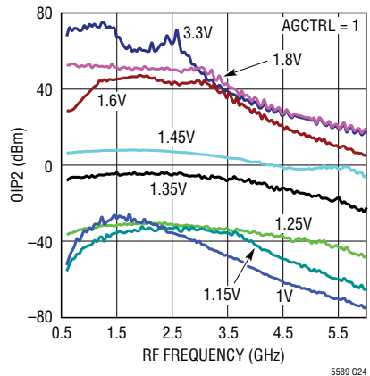
Output IP2 vs RF Frequency and V_{CTRL}
