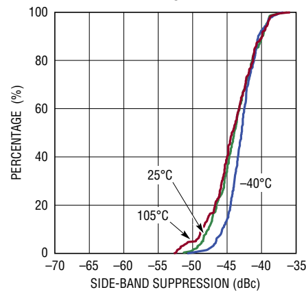
Side-Band Suppression Cumulative Distribution for V_{CTRL} = 1.75V
