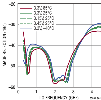
Image Rejection vs LO Frequency ( P_{LOM} = 10dBm )
