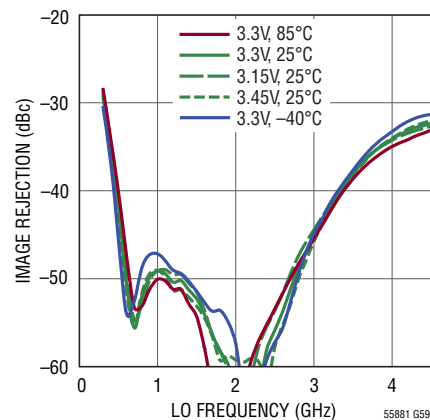
Image Rejection vs LO Frequency ( P_{LOM} = -5dBm )
