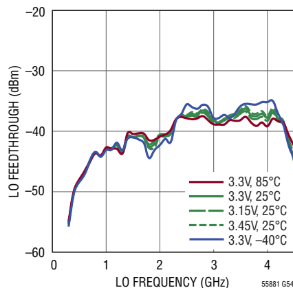
LO Feedthrough to RF Output vs LO Frequency ( P_{LOM} = -5dBm )
