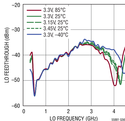
LO Feedthrough to RF Output vs LO Frequency ( P_{LOM} = 10dBm )
