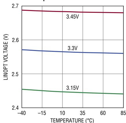
Floating LINOPT Voltage vs Temperature
