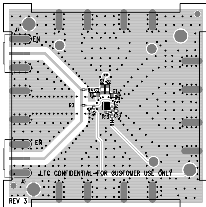
Figure 10. Bottom Side of Evaluation Board
