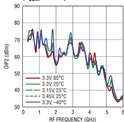
Output IP2 vs RF Frequency ( P_{LOM} = 0dBm )
