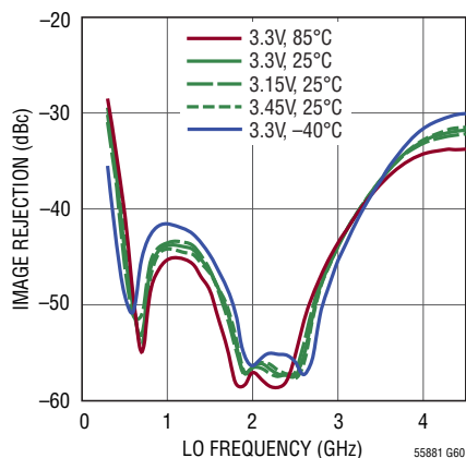
Image Rejection vs LO Frequency ( P_{LOM} = 5dBm )
