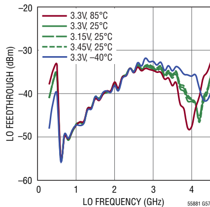
LO Feedthrough to RF Output vs LO Frequency ( P_{LOM} = 15dBm )
