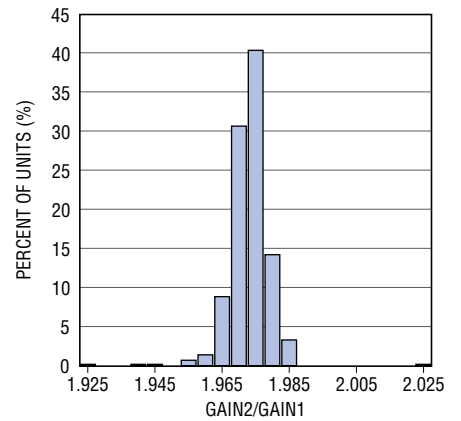
GAIN2/GAIN1 Histogram
