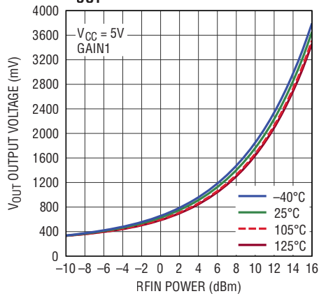
V_{OUT} vs Input Power 700 MHz
