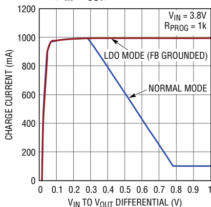
Charge Current vs ( V_{IN} - V_{OUT} ) Differential
