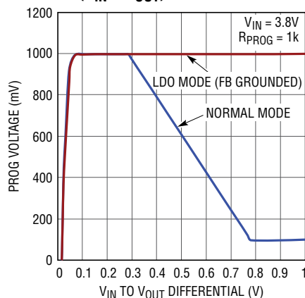
PROG Pin Voltage vs ( V_{IN} - V_{OUT} ) Differential
