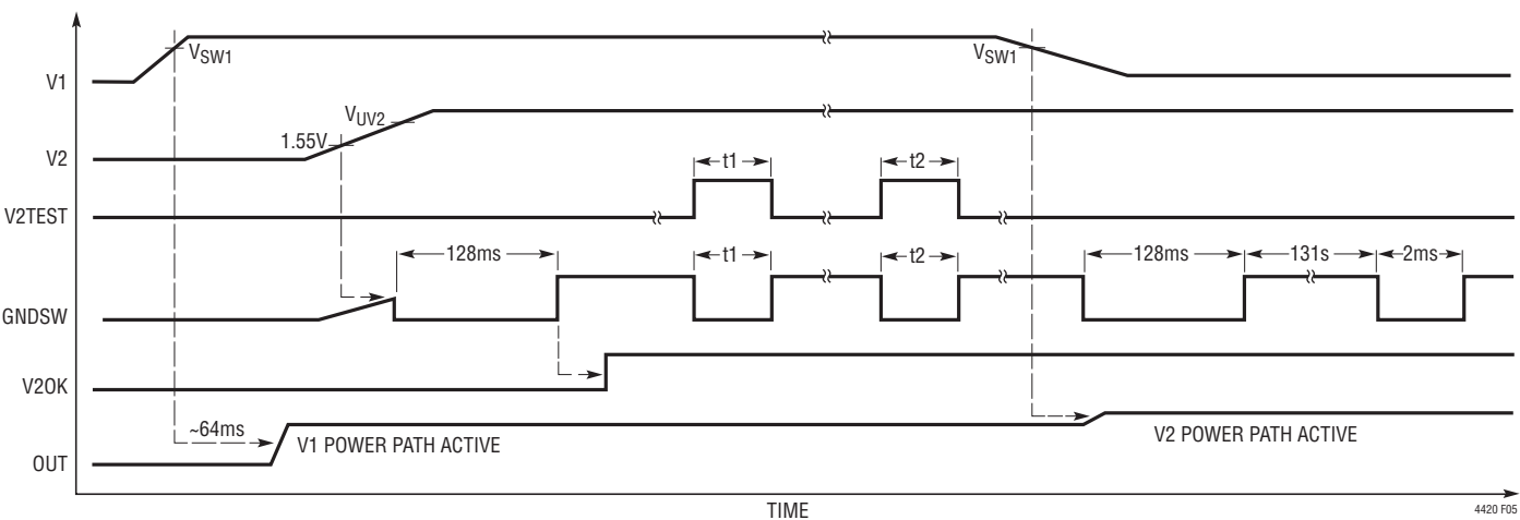
Figure 5. V2 Monitoring by Actively Driving VTEST. Note That t_1 and t_2 are < 128\text{ms}
