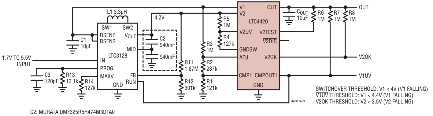
SuperCap Backup with SuperCap Charging
