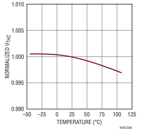
Normalized CMP1 and V2UV Falling Thresholds vs Temperature
