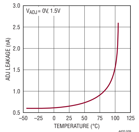
ADJ Leakage vs Temperature
