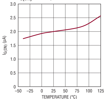
I_{G(\text{DN})} vs Temperature
