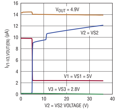
I_{V1-V3, V_{\text{OUT}}(\text{EN})} vs Supply Voltage
