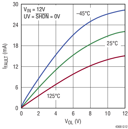
\overline{\text{FAULT}} Output Current vs Voltage
