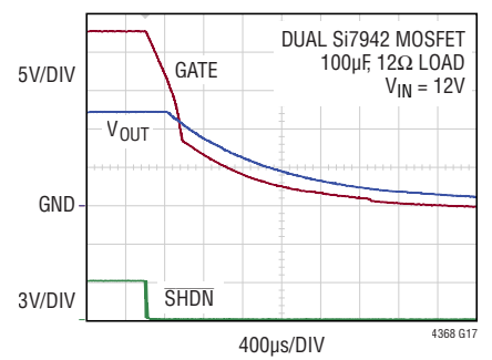
Turn-Off Timing
