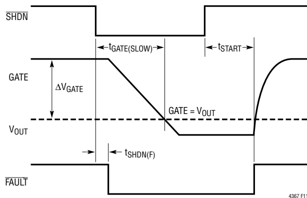
Figure 11. Shutdown Timing
