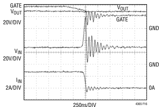
Figure 16. Transients During OV Fault When No Transorb (TVS) Is Used
