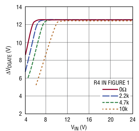
\Delta V_{DGATE} vs V_{IN} in Figure 1
