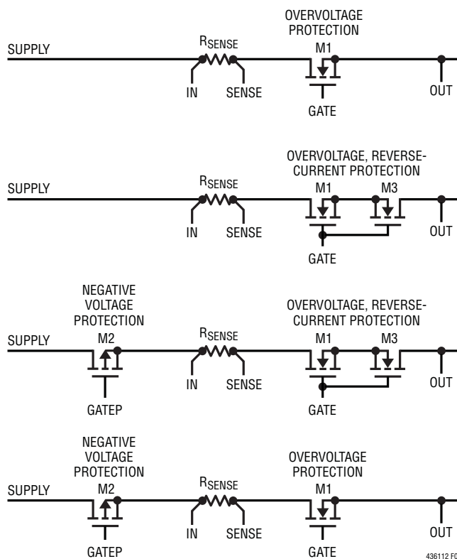
Figure 3. MOSFET Configurations
