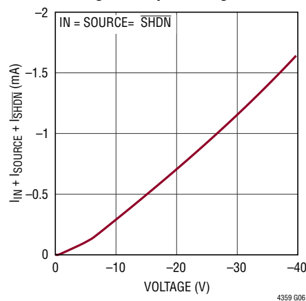
Total Negative Current vs Negative Input Voltage
