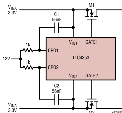
Figure 3. 3.3V Ideal Diode with External 12V Supply Powering CPO for Faster Start-Up and Refresh
