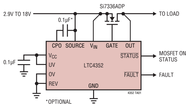
2.9V to 18V Ideal Diode
