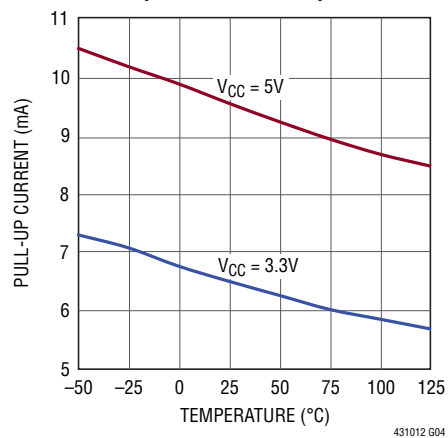
SDA, SCL Rise Time Accelerator Pull-Up Current vs Temperature
