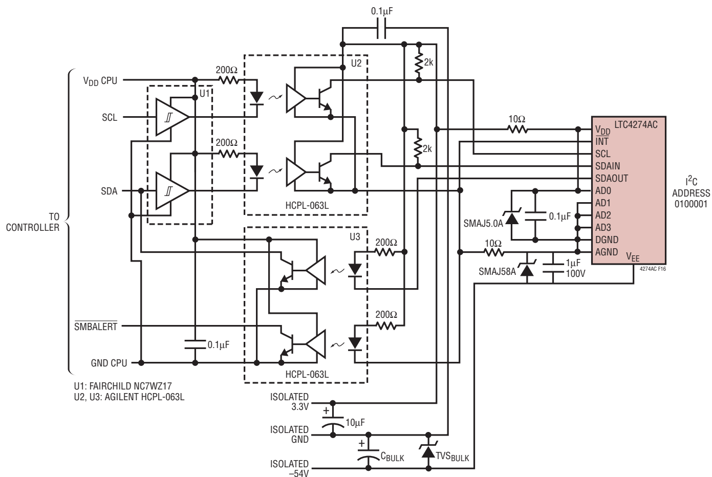
Figure 16. Opto-Isolating the I²C Bus
