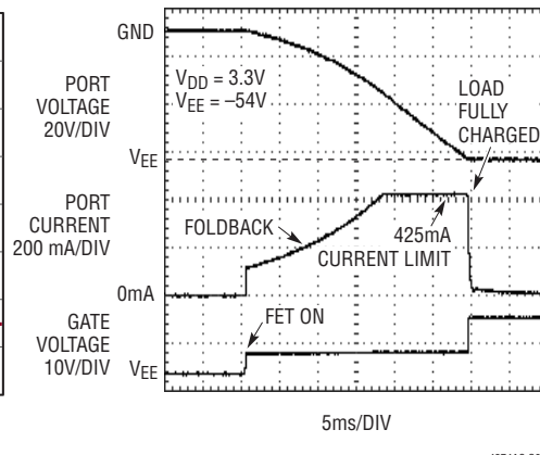
Powering Up into a 180 \mu F Load
