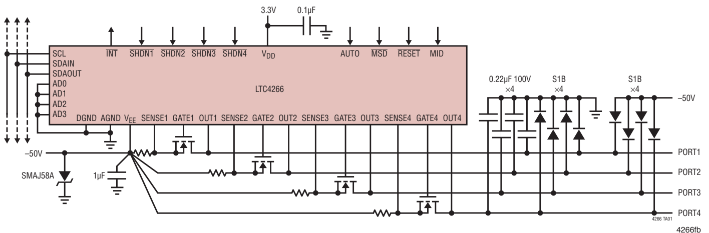
Complete 4-Port Ethernet High Power Source
