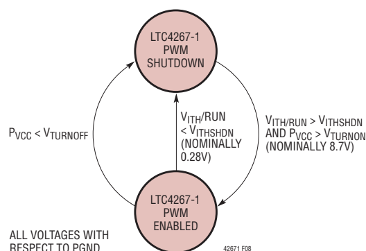
Figure 8. LTC4267-1 Switching Regulator Start-Up/Shutdown State Diagram
